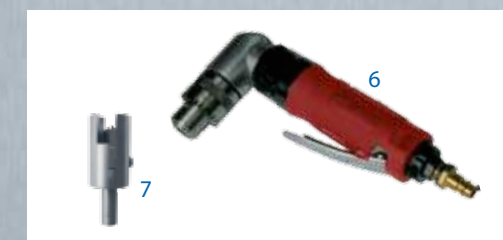
Fig. 6 Special electrode cap milling machine for quick and easy copy-milling of electrode caps incl. tip dresser (fig. 7)
